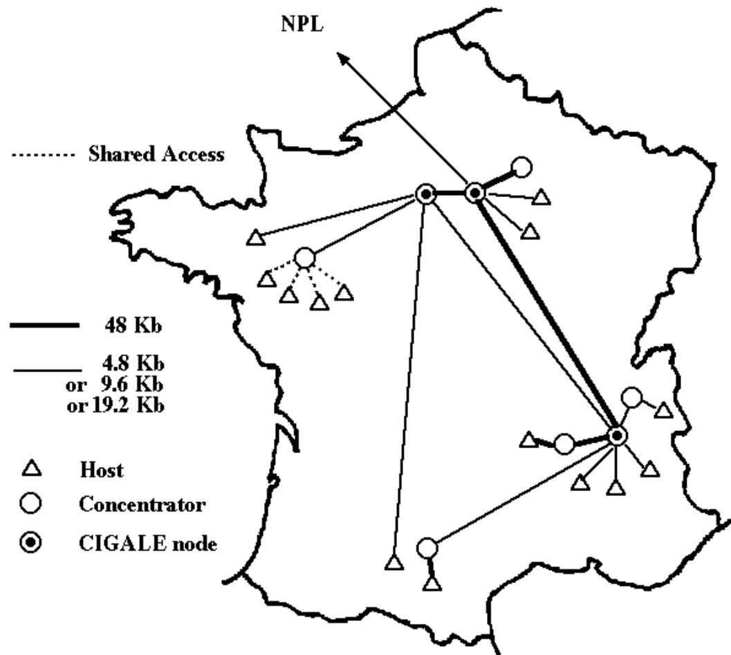
FIG. 1. - CYCLADES topology
